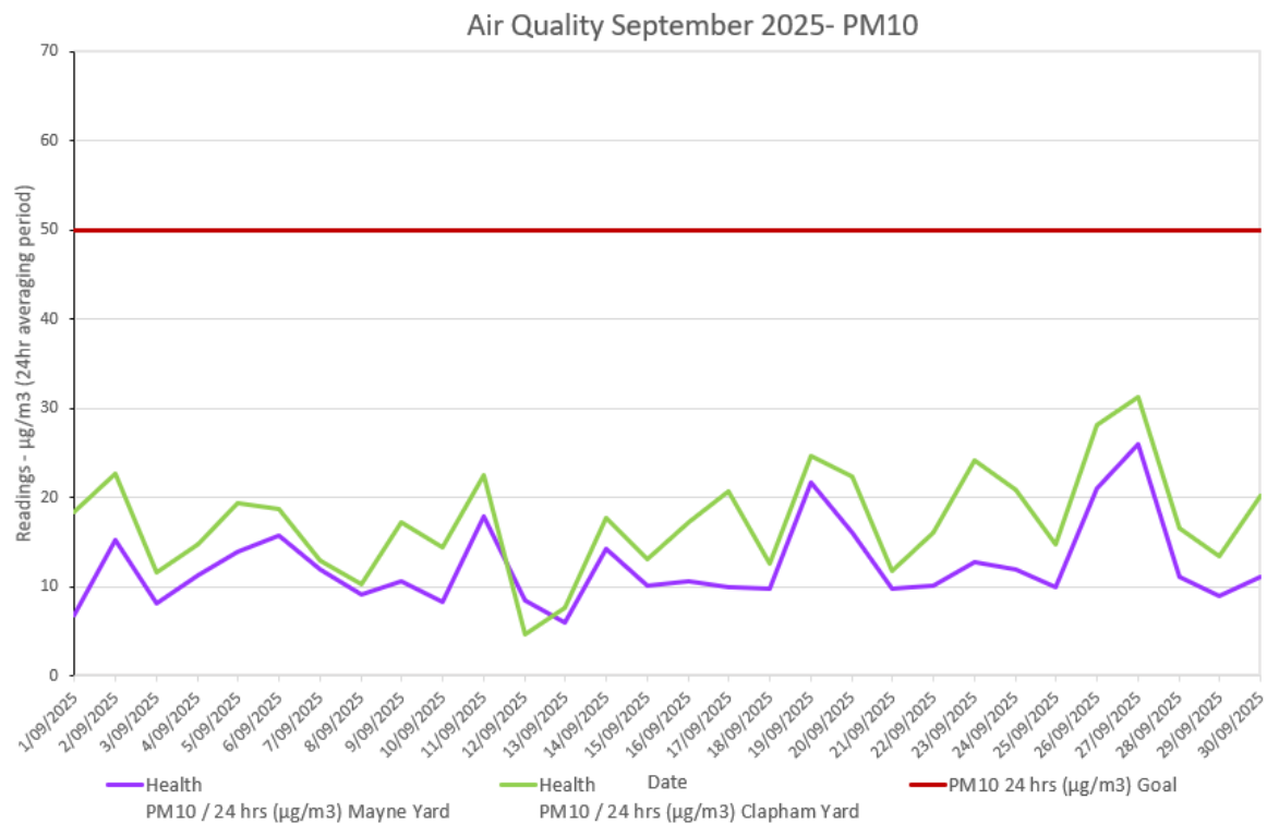
Figure 3: Air Quality Monitoring - PM10 Data
