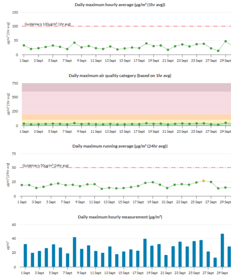
Figure 3: Woolloongabba – DETSI Station - PM10 graph for September 2025 (reproduction from the DETSI website).
